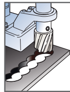
Overlapped cutting
