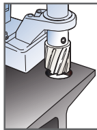
Cutting in H-beams
